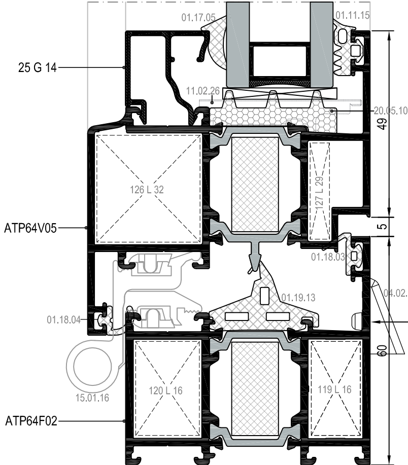
⑥ DETAYI DETAIL
